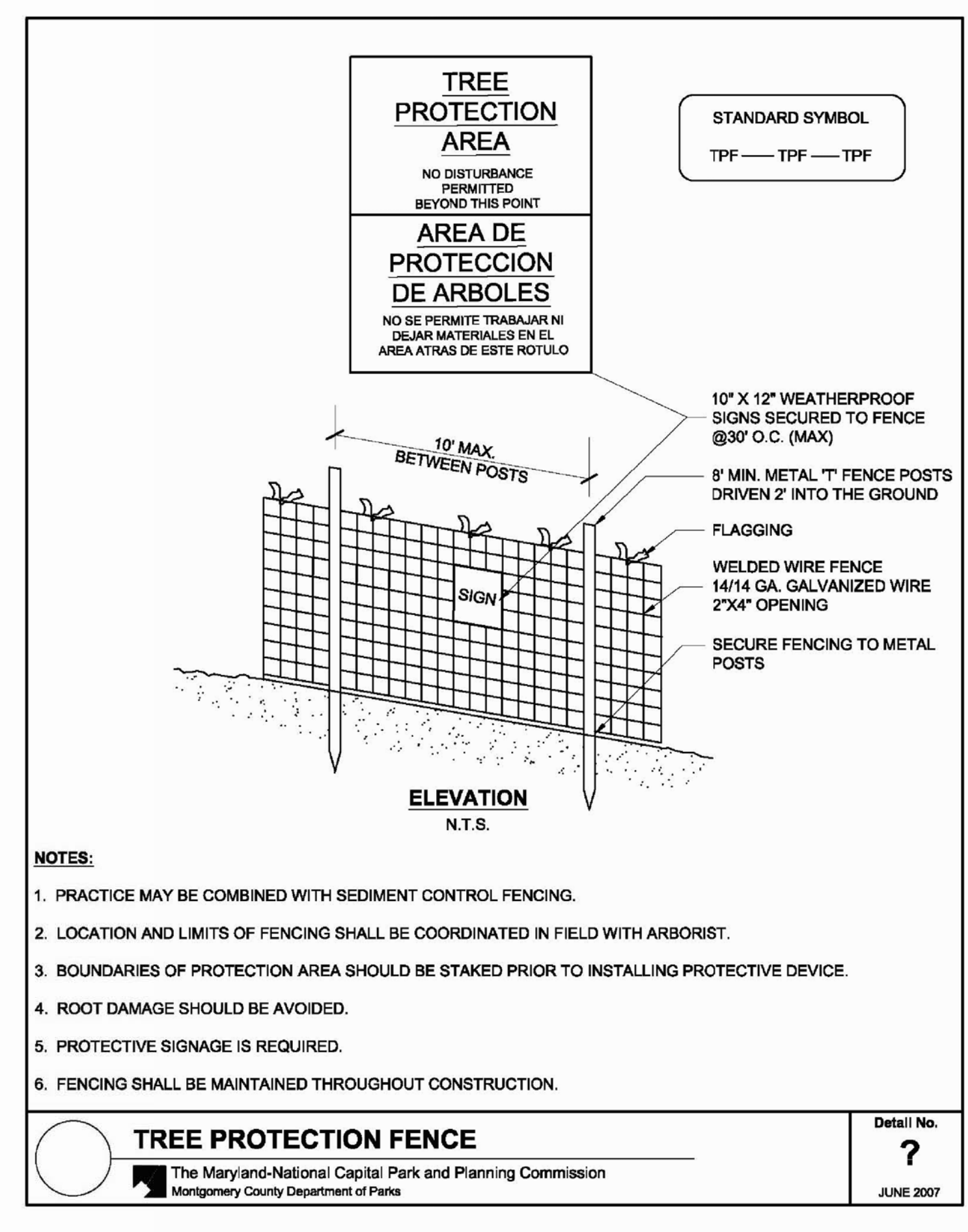
1 A-2 TREE PROTECTION FENCE SCALE: NTS
