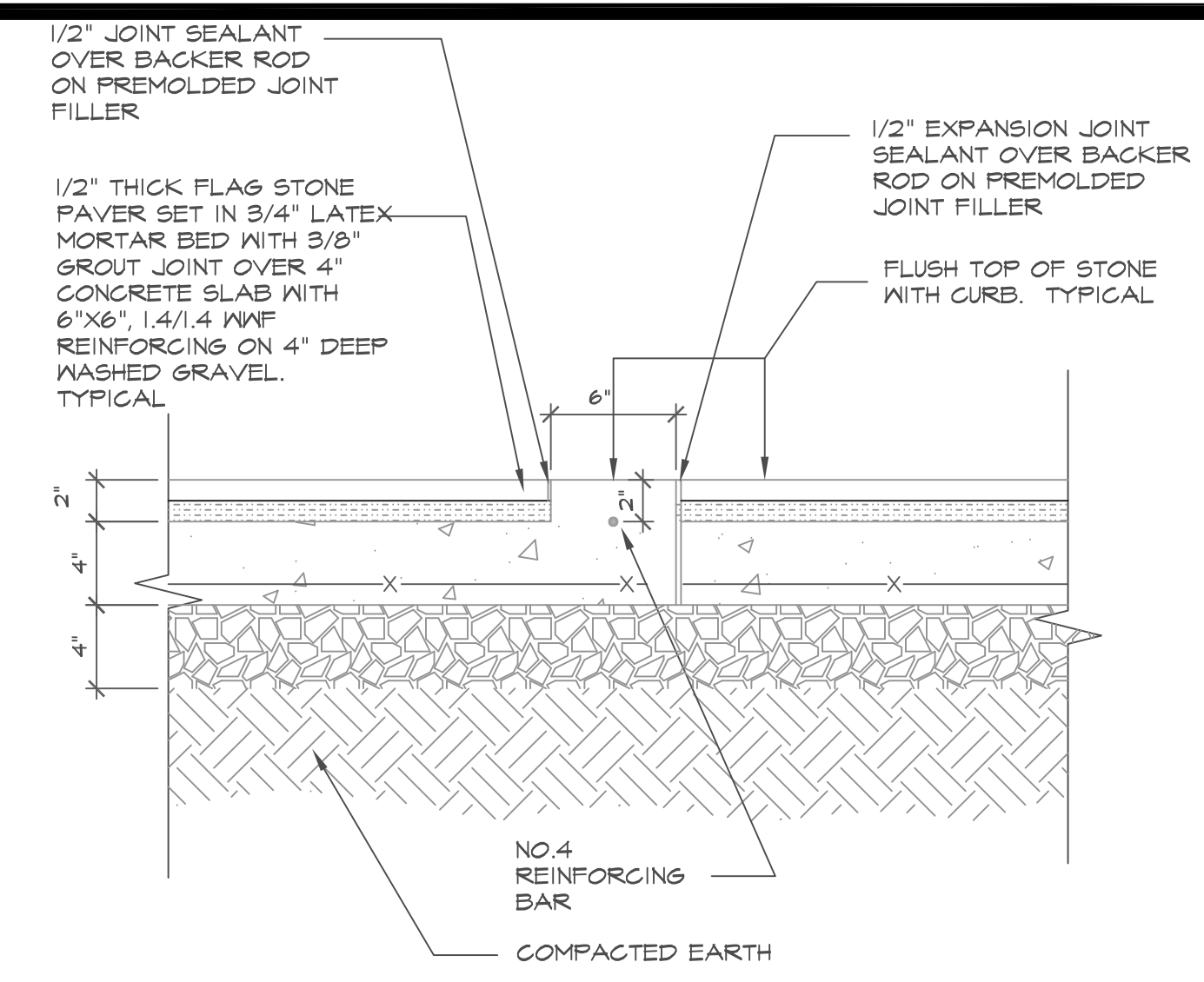
2 DETAIL AT CURB SCALE: 1 1/2" = 1'-0"
